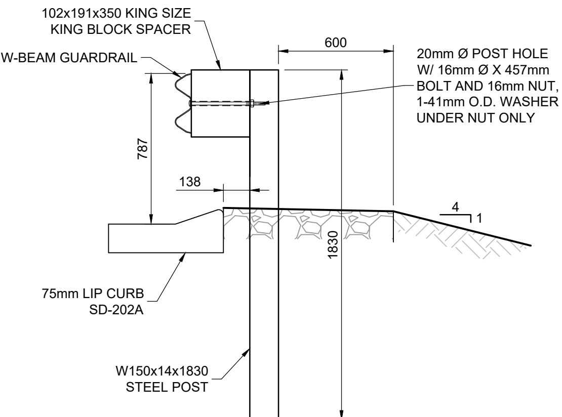
B - - 1:20 MIDWEST GUARDRAIL SECTION
