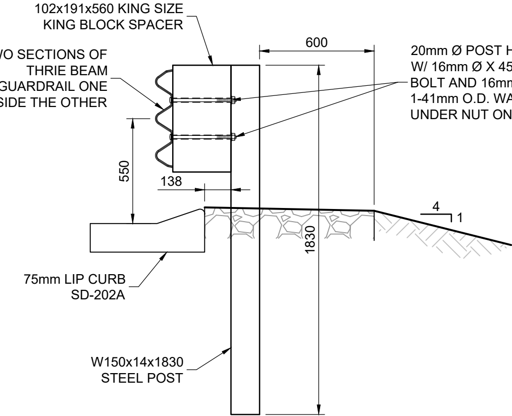
A - - 1:20 APPROACH GUARDRAIL SECTION
