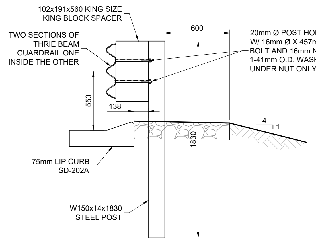
A - - APPROACH GUARDRAIL SECTION 1:20
