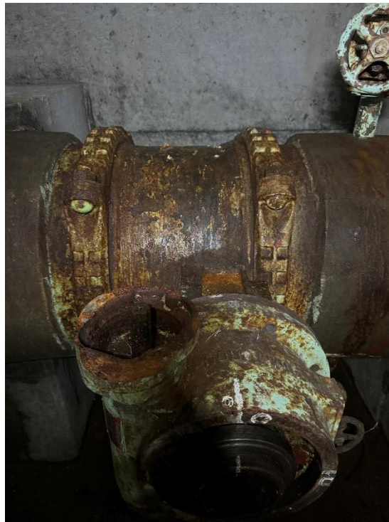
Figure 19: North Valve Chamber Existing Valve with Broken Operator
