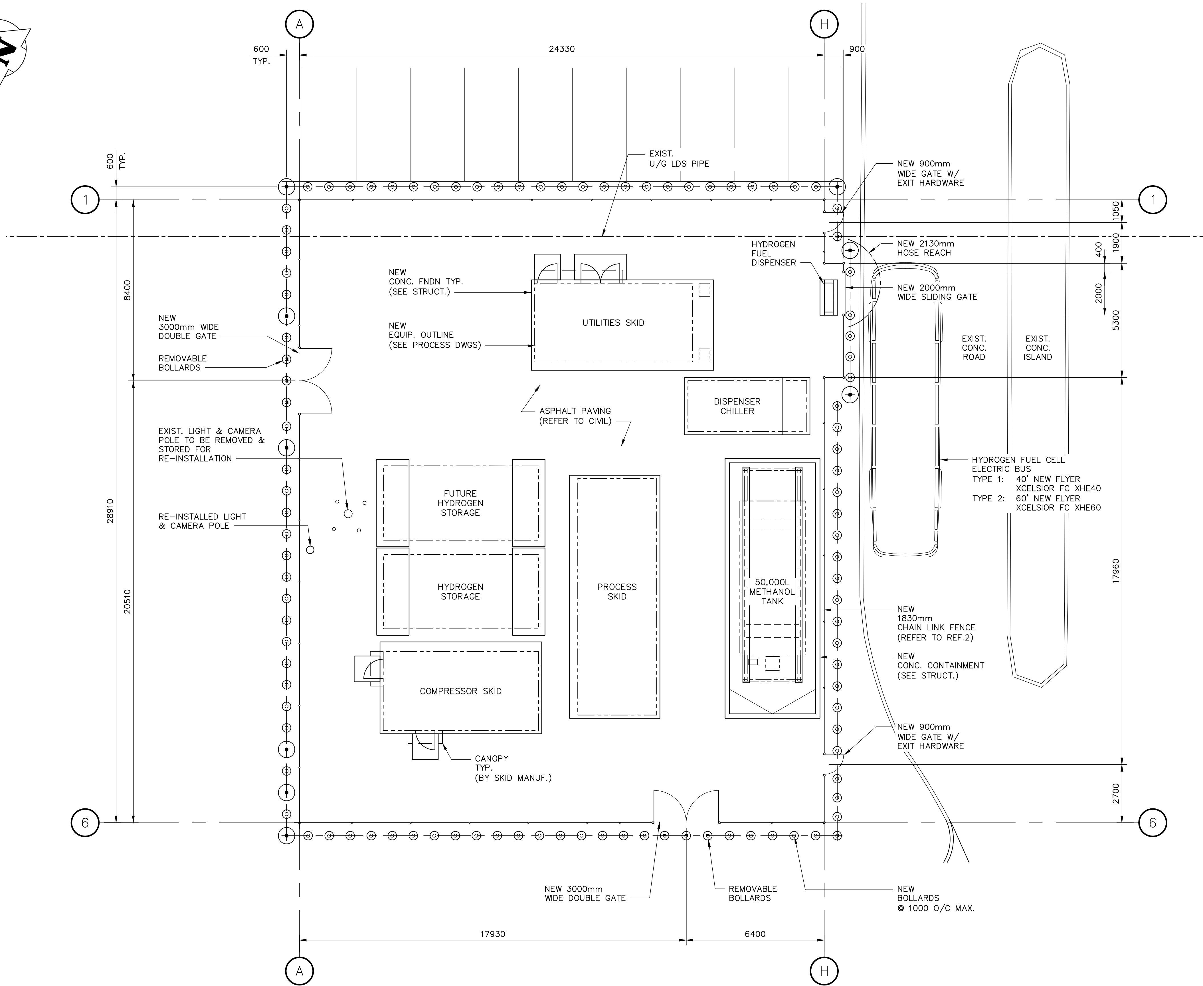
1 GENERAL ARRANGMENT PLAN REF.1 SCALE: 1:100
