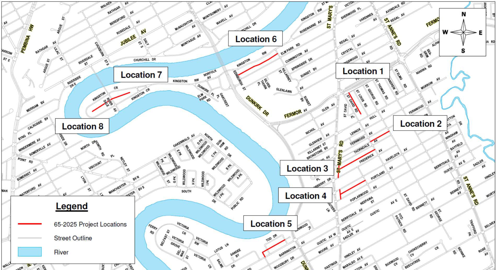
65-2025 Cement Stabilization of Gravel Back Lanes Map 1 of 2
