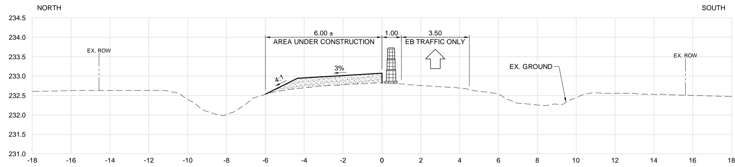
TYPICAL RESURFACING SECTION - STAGE 1 (STA. 1+300 SHOWN) SCALE: H = 1:100, V = 1:50
