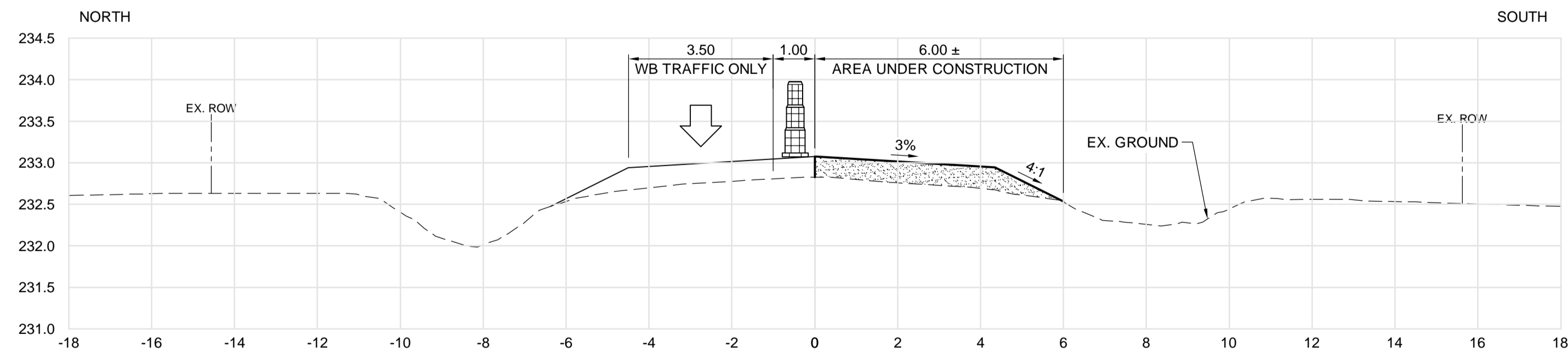
TYPICAL RESURFACING SECTION - STAGE 2 (STA. 1+300 SHOWN) SCALE: H = 1:100, V = 1:50
