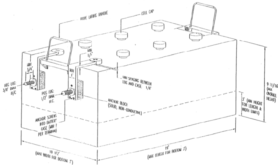
BUS BATTERY WITH DROP TERMINALS -- Dimensional Specifications --
