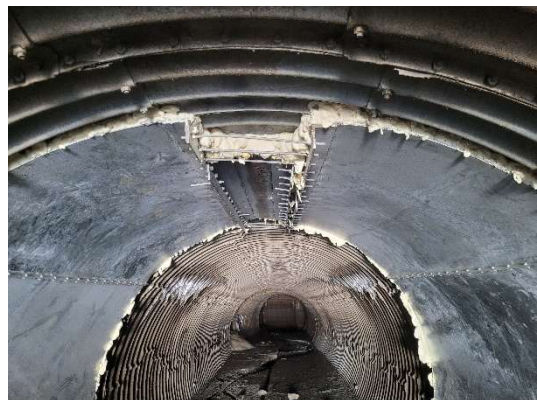
Photo 12: Roland Outfall – Emergency repair/slip joint. Looking upstream towards 1350 SRS connection and chamber
