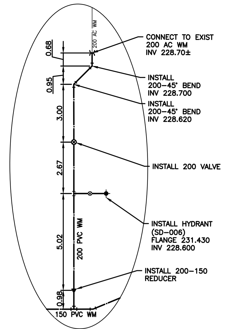
DETAIL "A" SCALE : NTS
