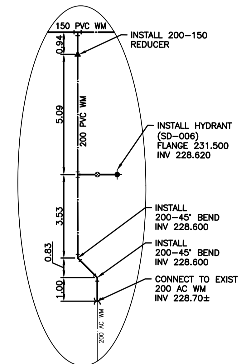
DETAIL "B" SCALE : NTS
