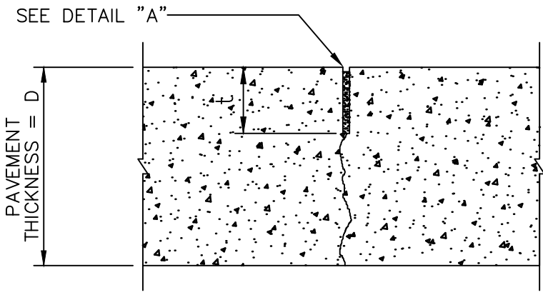
SAWN JOINT
