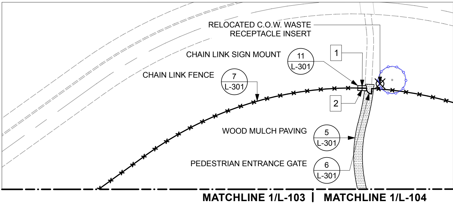
2 NORTH MATERIALS, LAYOUT, SITE FURNISHING & PLANTING PLAN Scale: 1:500
