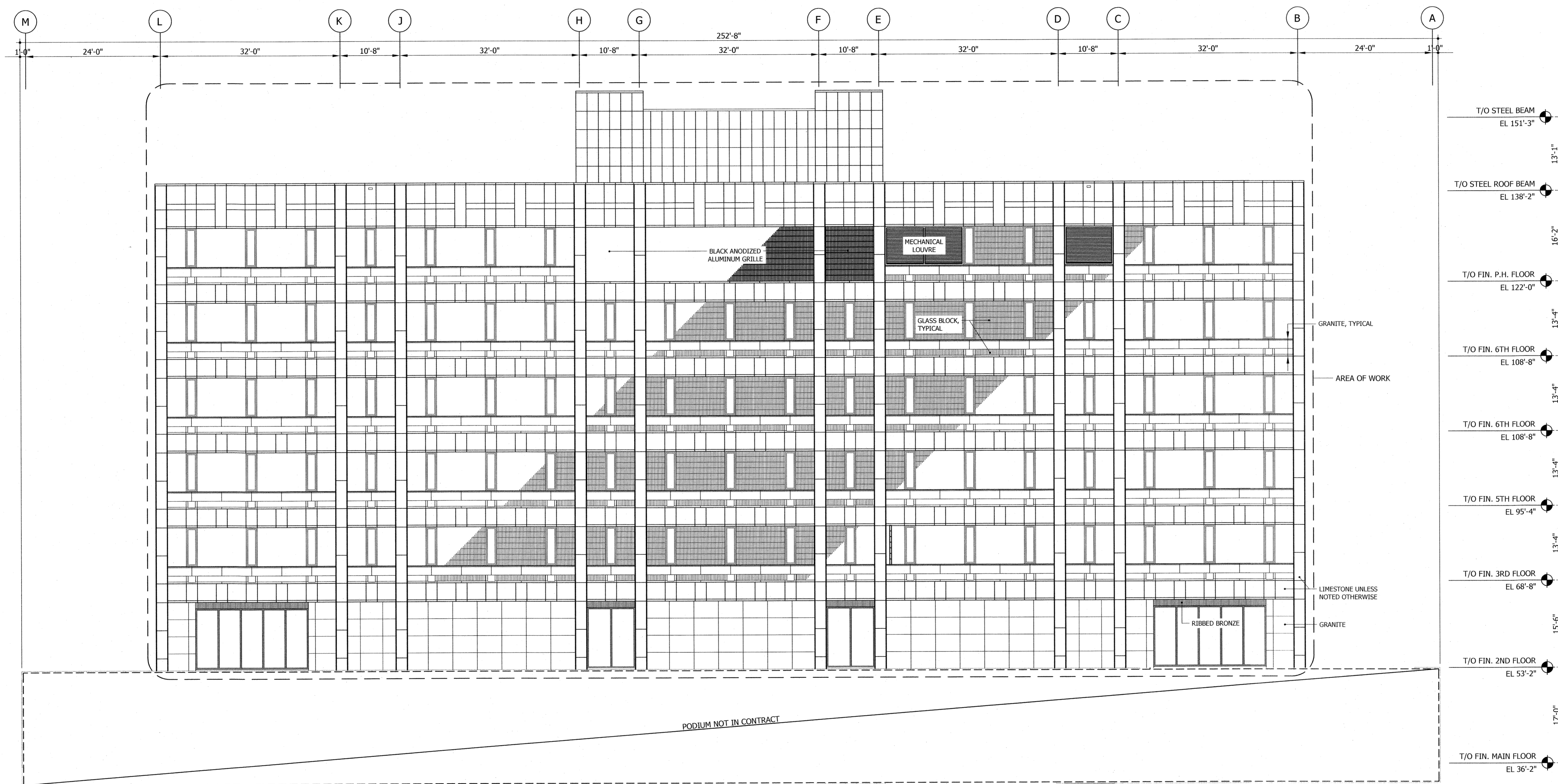
1 NORTH ELEVATION S0.1 | S3.1 | 3/32" = 1'-0"
