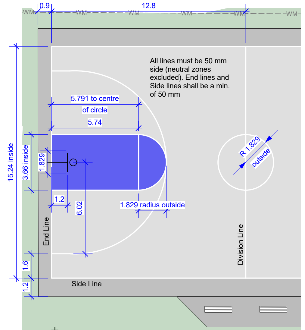
1 Basketball Court Enlargement Scale: 1:150
