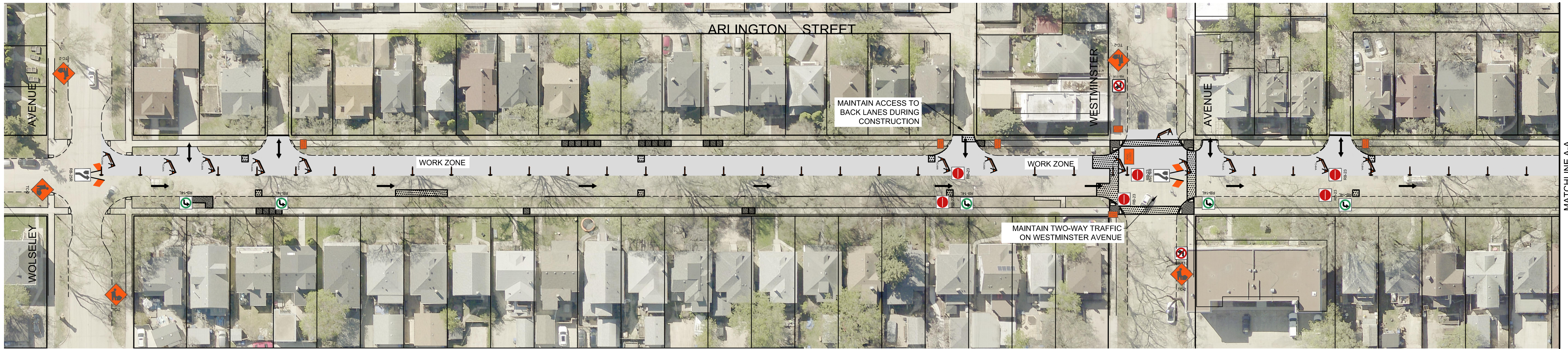
PLAN - STAGE 1 Scale 1:500
