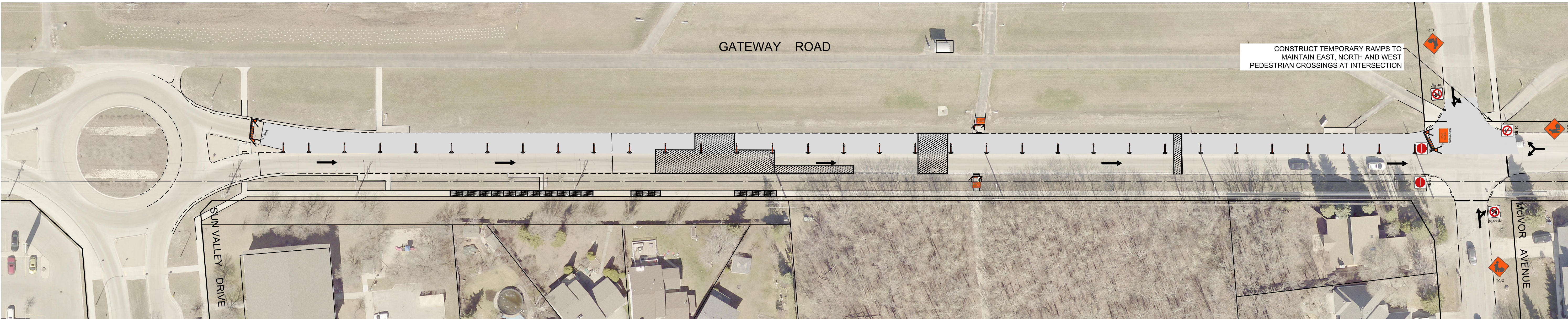
PLAN - STAGE 1 Scale 1:500
