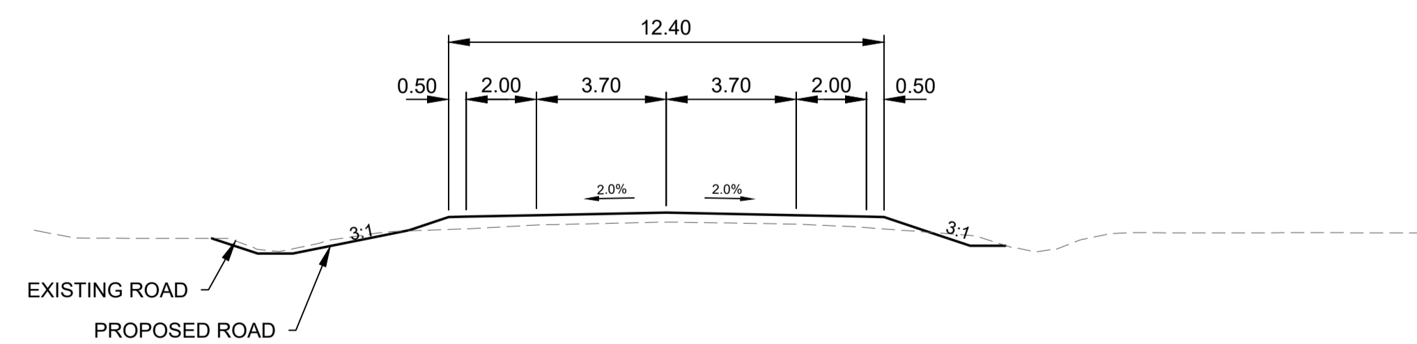
CROSS-SECTION - STATION 2+30 SCALE 1:150
