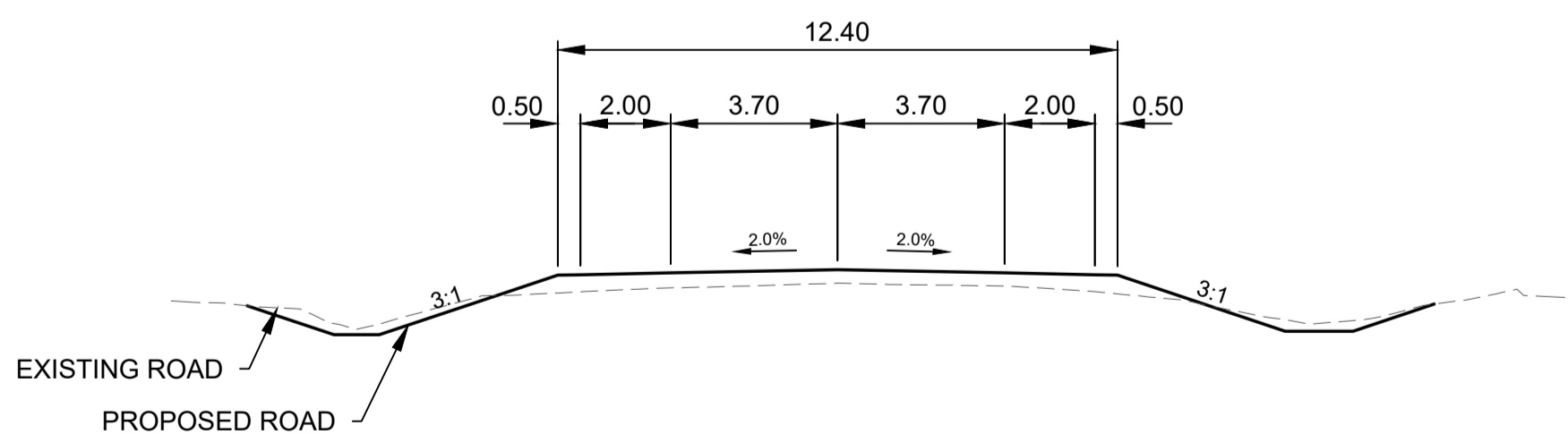
CROSS-SECTION - STATION 14+00 SCALE 1:150
