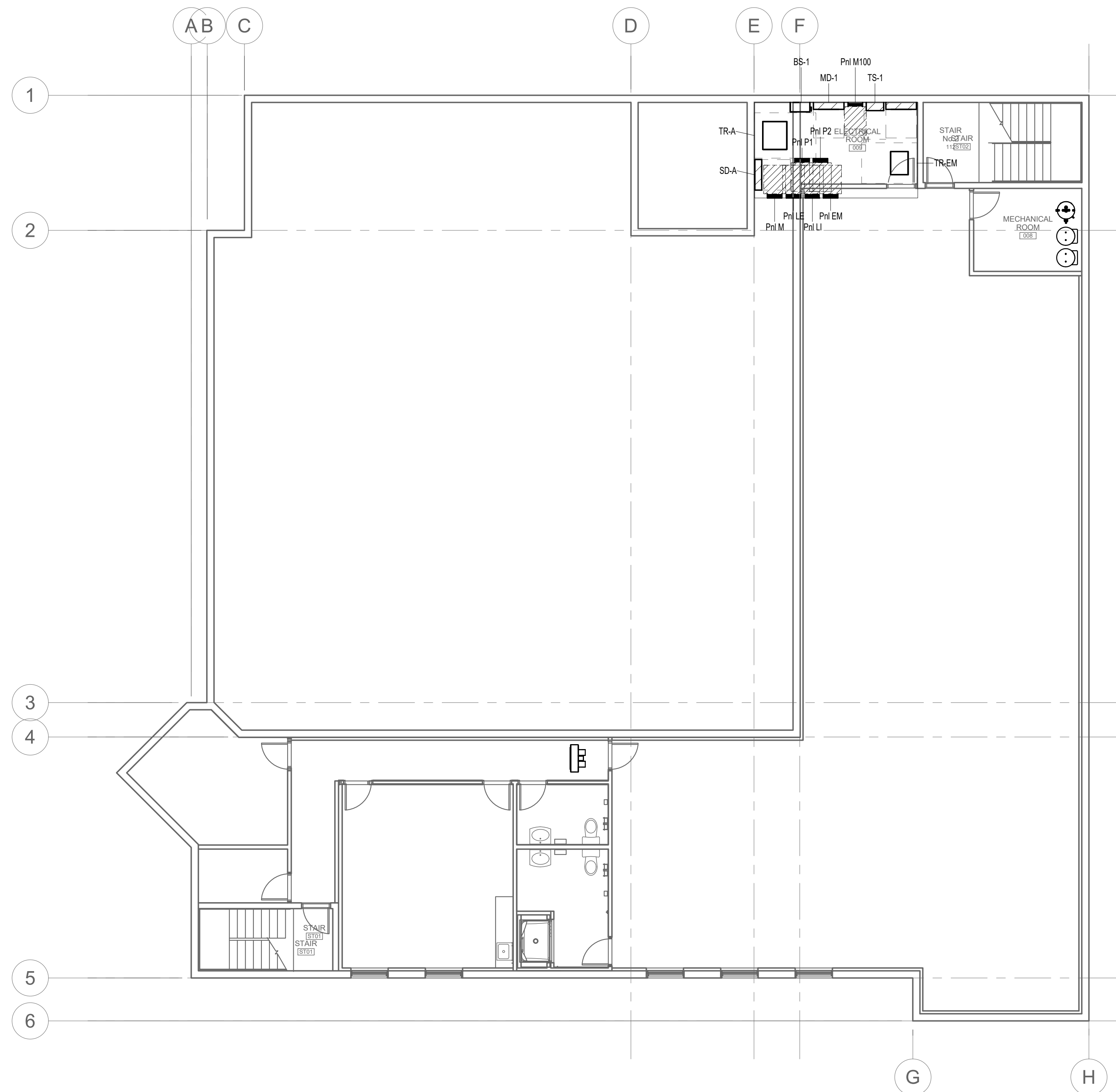
1 BASEMENT FLOOR PLAN - POWER & SYSTEMS EP2.0 SCALE: 1 : 100
