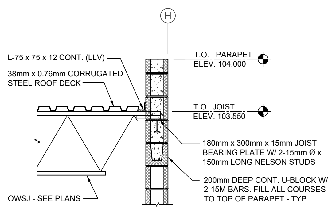
8 SECTION S5/S6 SCALE = 1:20
