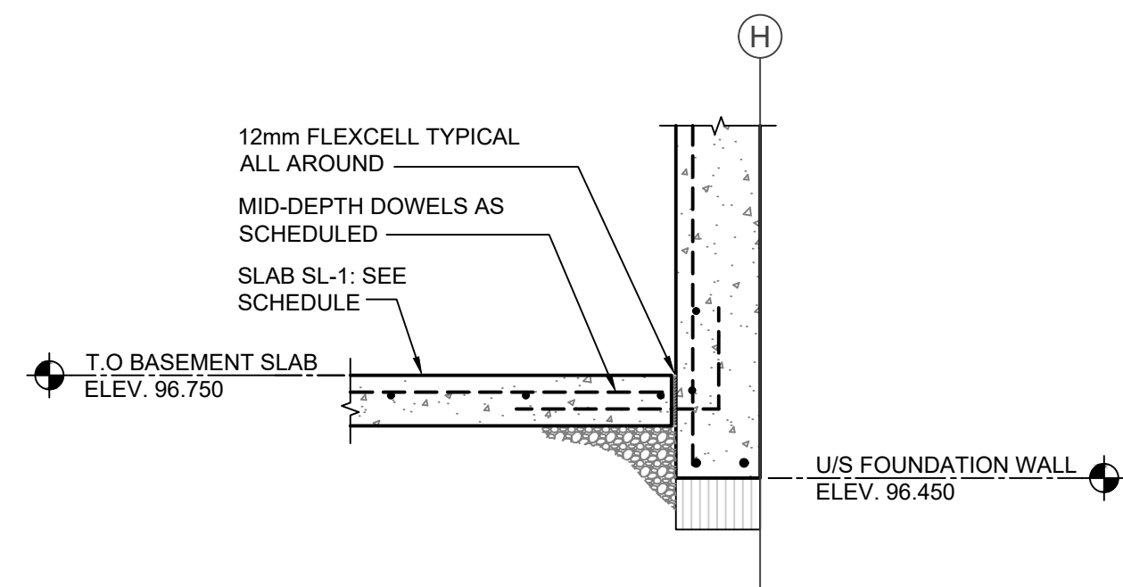
5 SECTION S2/S6 SCALE = 1:20
