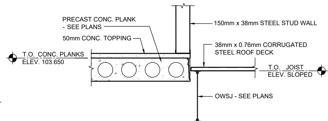
6 SECTION S4/S6 SCALE = 1:20
