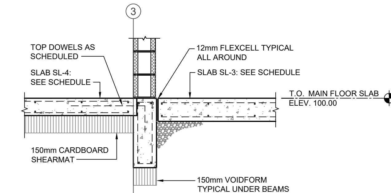
12 SECTION S3/S6 SCALE = 1:20
