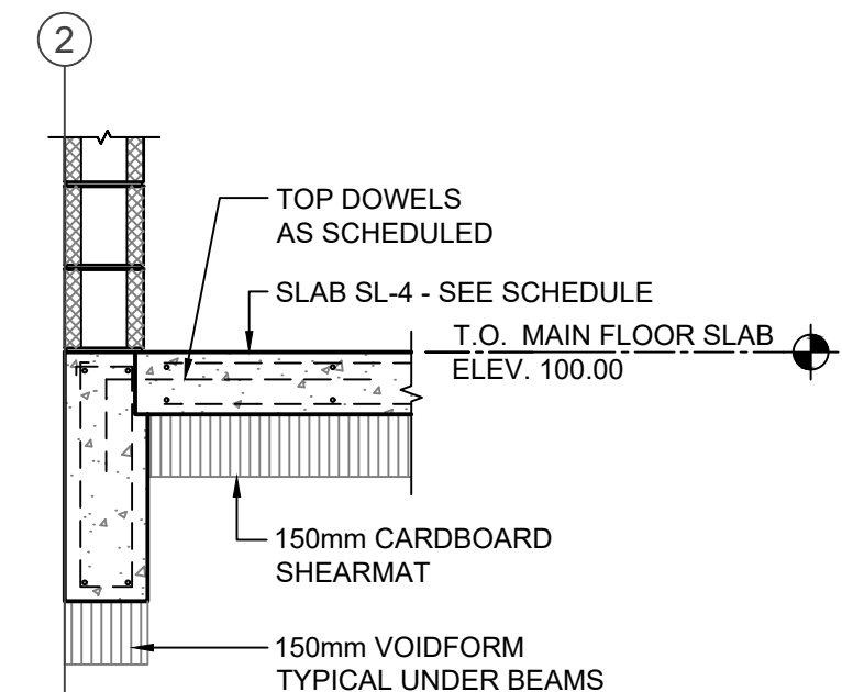
11 SECTION S3/S6 SCALE = 1:20
