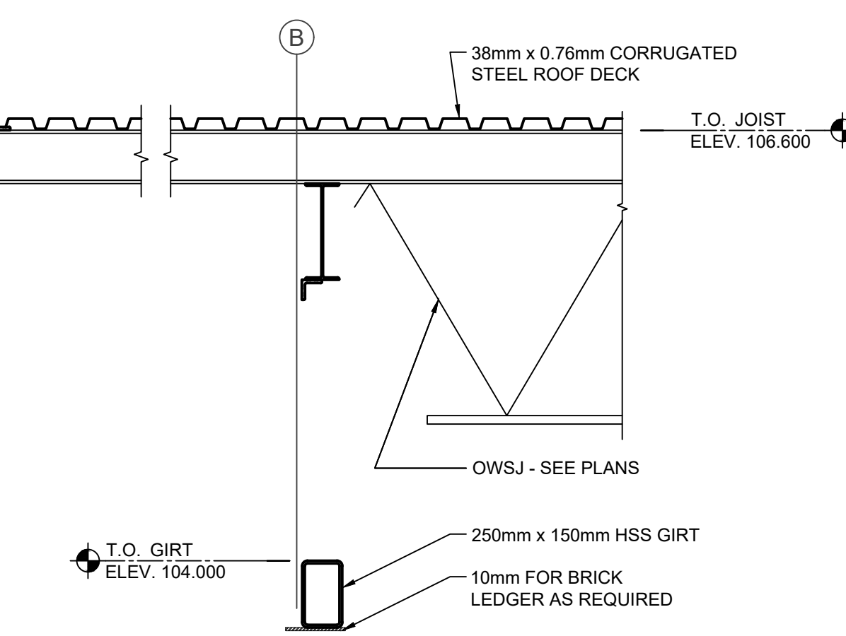
13 SECTION S3/S6 SCALE = 1:20
