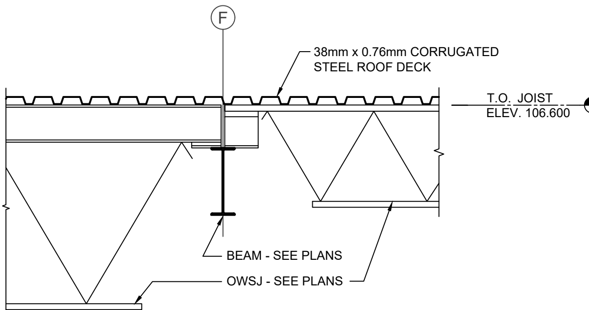
9 SECTION S5/S6 SCALE = 1:20
