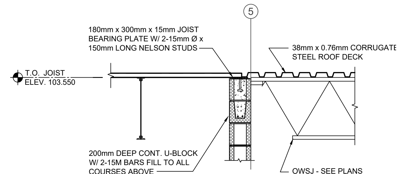
10 SECTION S4/S6 SCALE = 1:20
