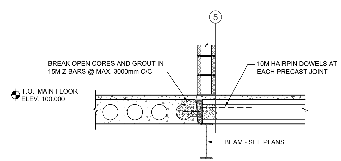
14 SECTION S3/S6 SCALE = 1:20
