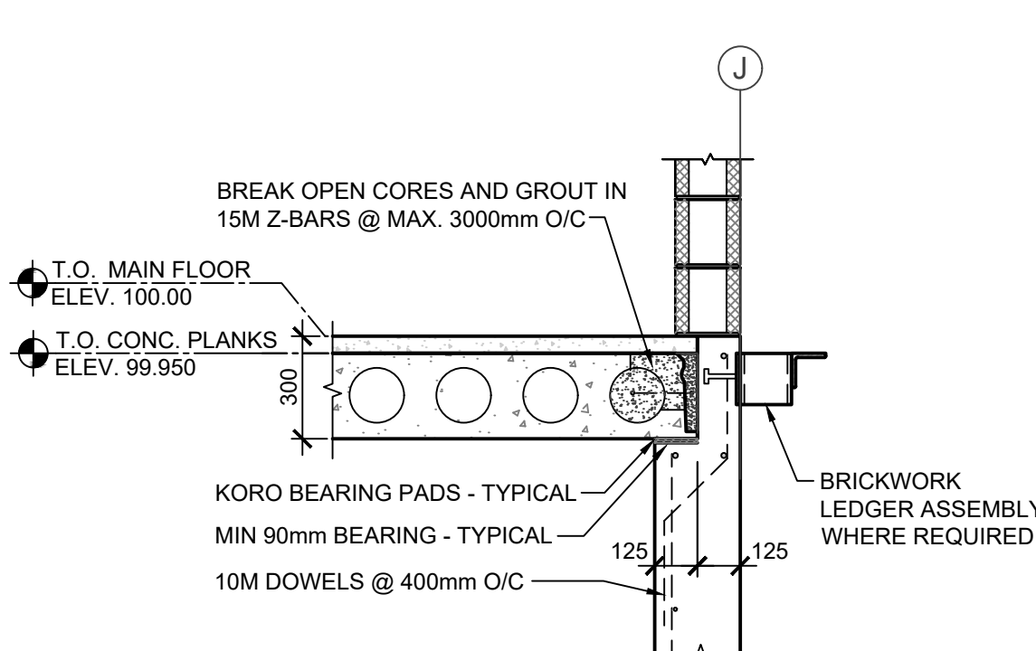
15 SECTION S3/S6 SCALE = 1:20
