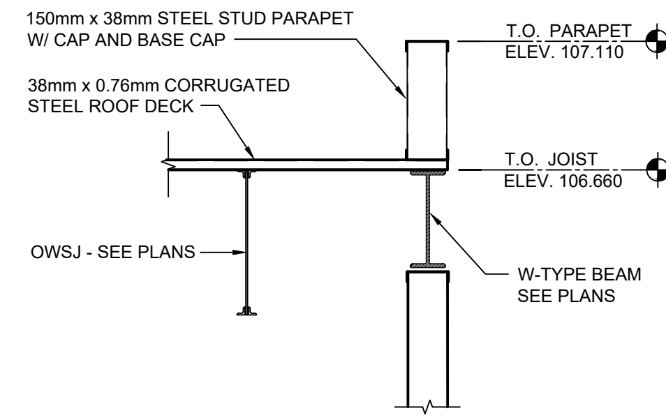
2 SECTION S5/S6 SCALE = 1:20
