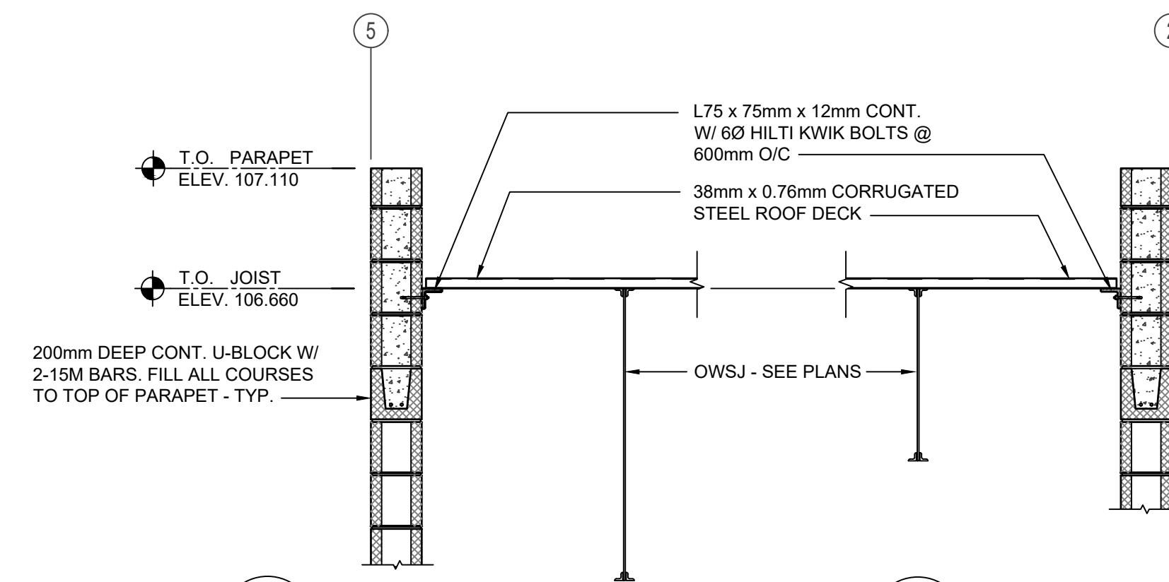
3 SECTION S5/S6 SCALE = 1:20
