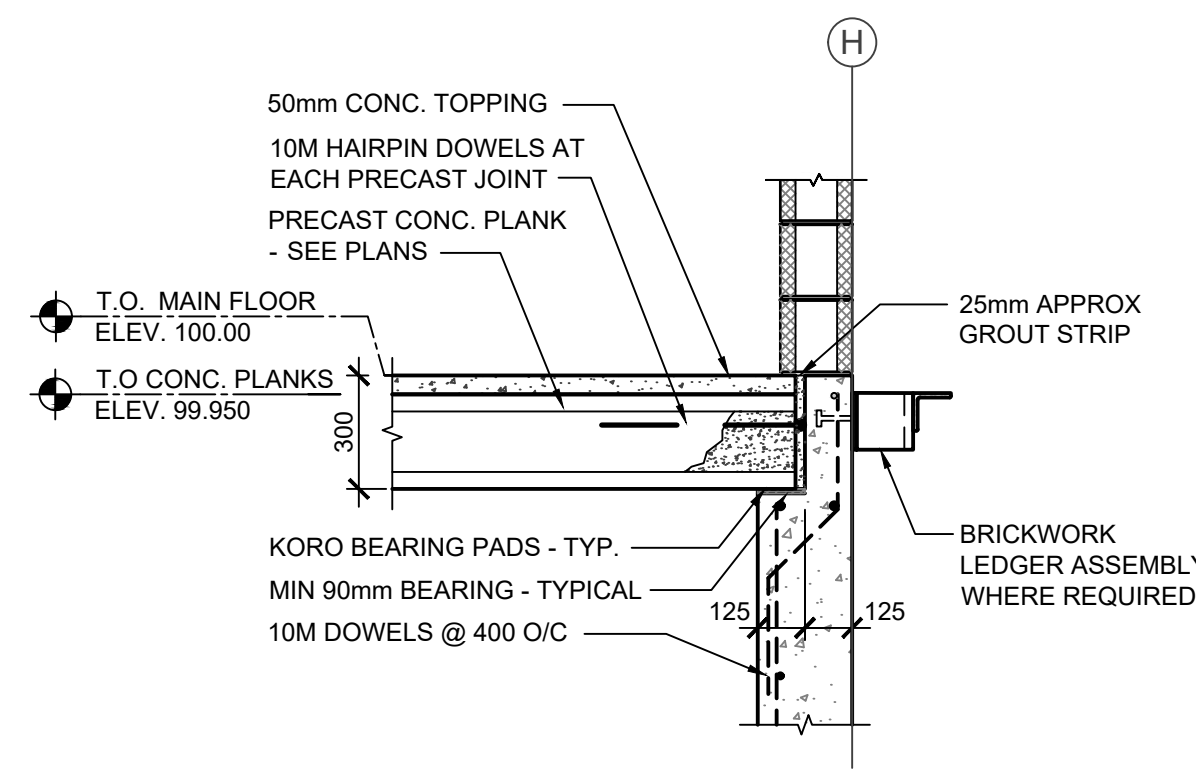
1 SECTION S3/S6 SCALE = 1:20
