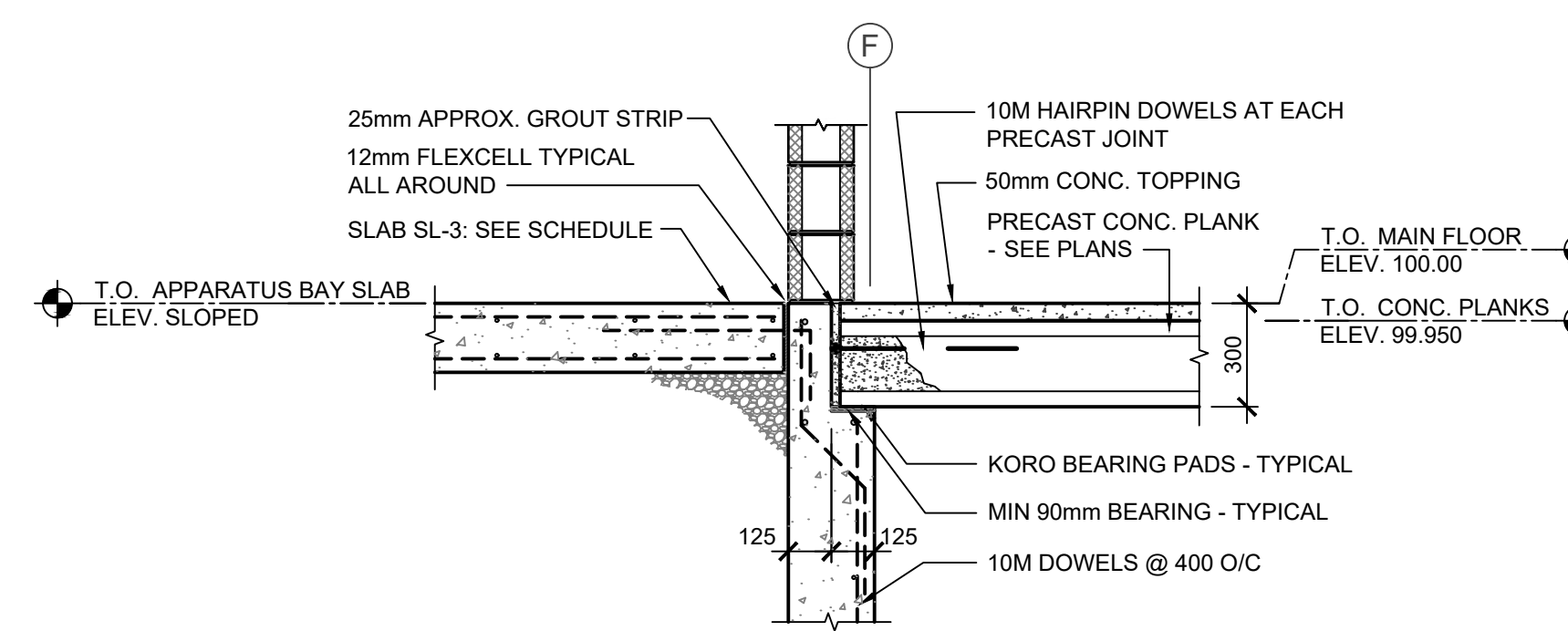
7 SECTION S3/S6 SCALE = 1:20
