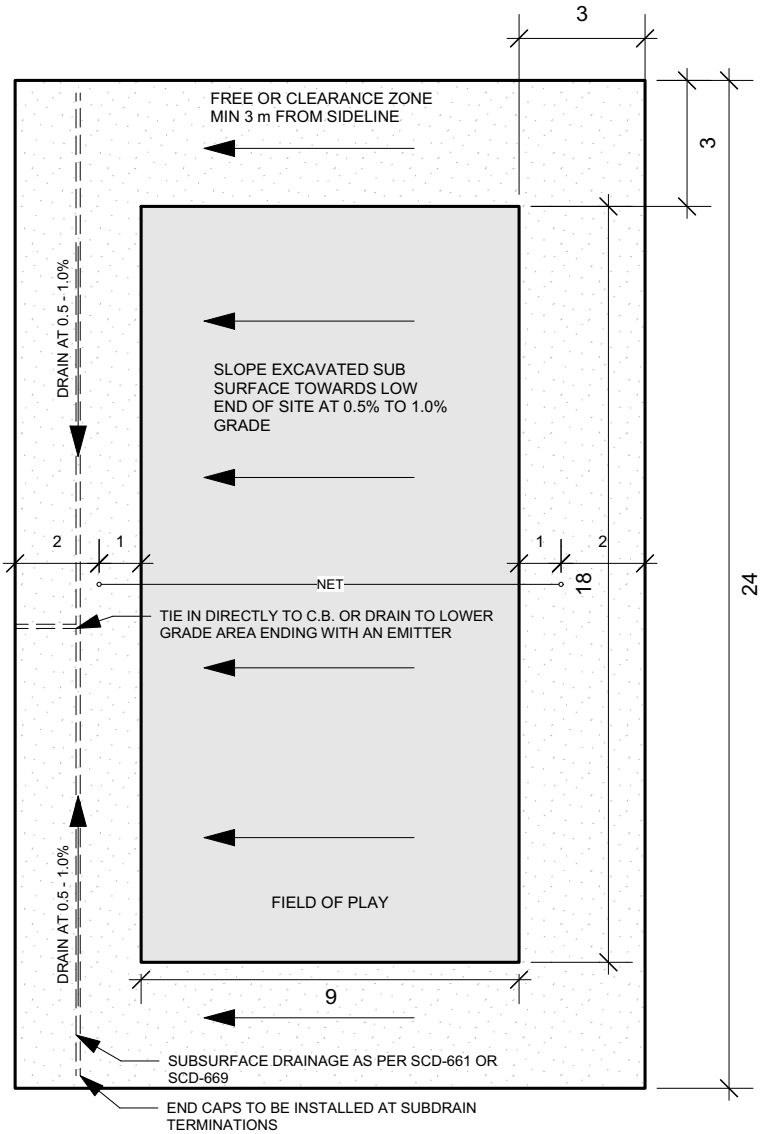
BEACH VOLLEYBALL COURT DIMENSIONS SCALE: 1:180
