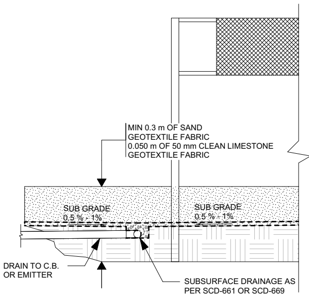
SUBDRAIN DETAIL SCALE: 1:50
