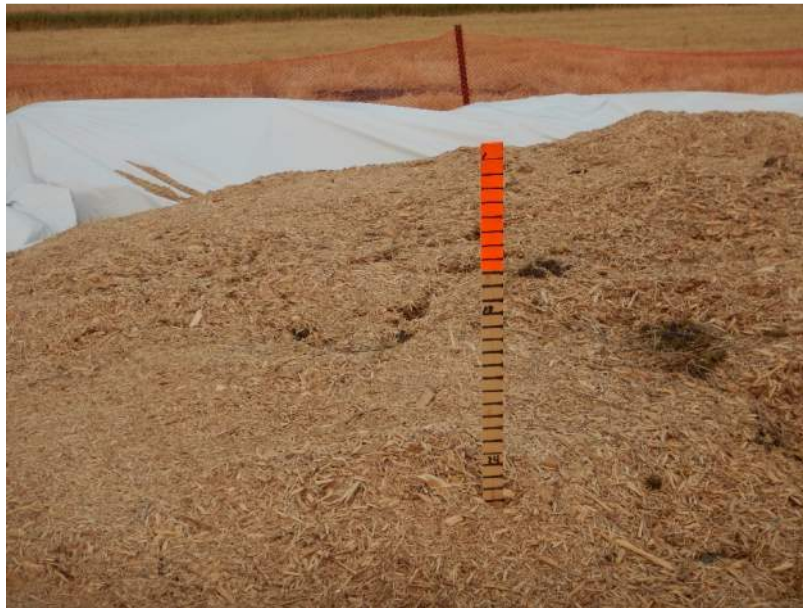
Photograph 2. Wooden stake used to measure degree of slumping of biosolids stockpiles.
